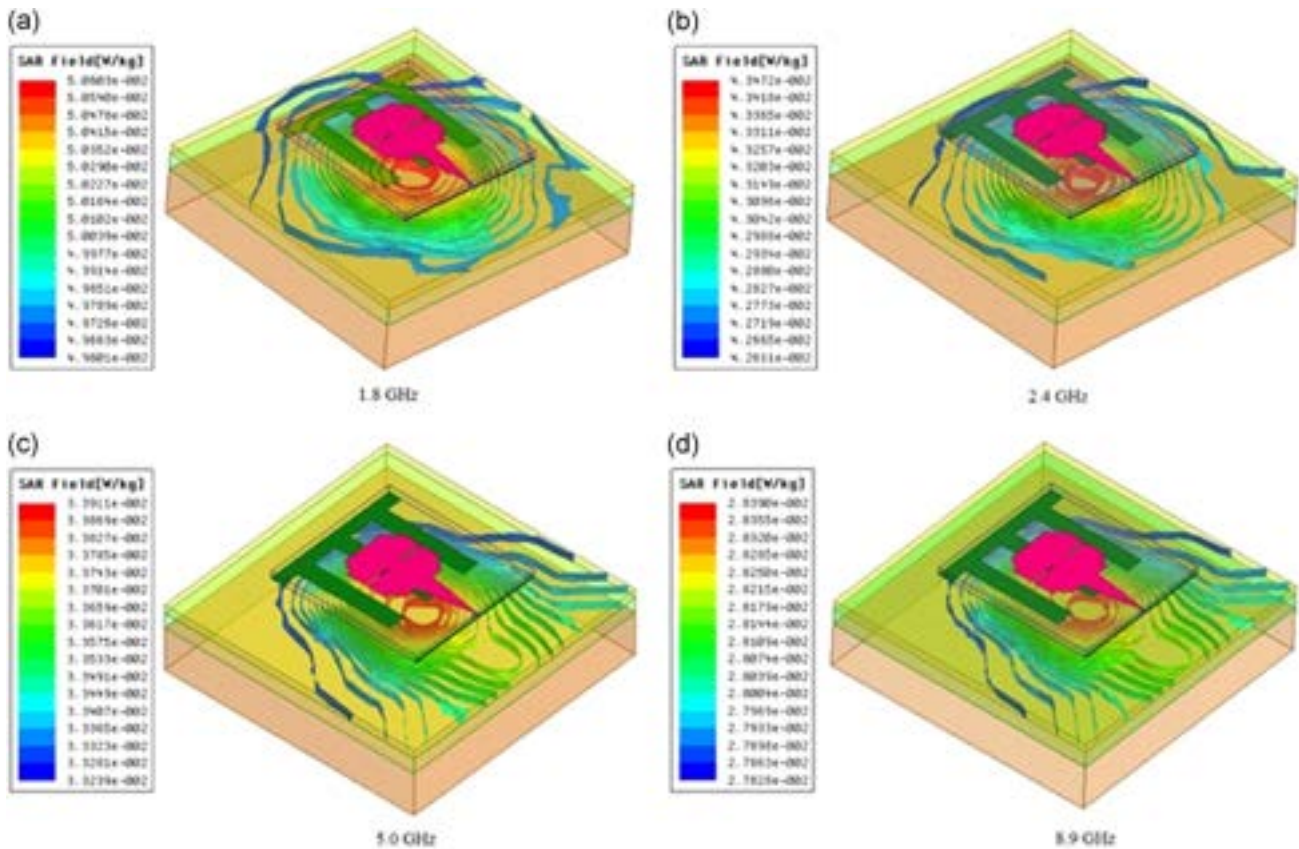
Fig. 4. Corresponding specific absorption rate ( SAR_{1g} ) distribution of the patch antenna shown in Figure 3, where the maximum SAR occurs at the location of the greatest maximum field amplitude for (a) 1.8 GHz, (b) 2.4 GHz, (c) 5.0 GHz, and (d) 8.9 GHz [Karthik and Rao, 2018].
